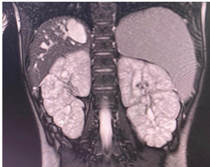
Fig. 3. MRI in coronal section, balanced in T2: highlighting globular kidneys, site of multiple cystic formations of the medulla, realizing a sponge appearance. Presence of a major cystic and moniliform dilatation of the intrahepatic bile ducts falling within the scope of Cacchi-Ricci disease
