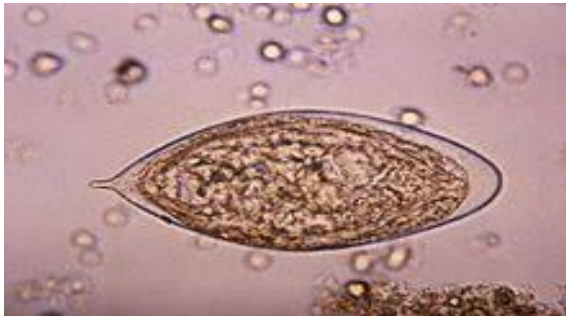
Fig. 1. Shows Schistosoma haematobium Ova in urine
