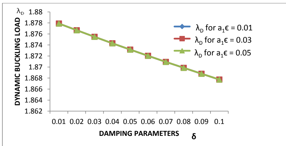
Fig. 2. Relationship between the dynamic buckling load and the damping factors for different values of Imperfection Parameters, using equation (4.122)
