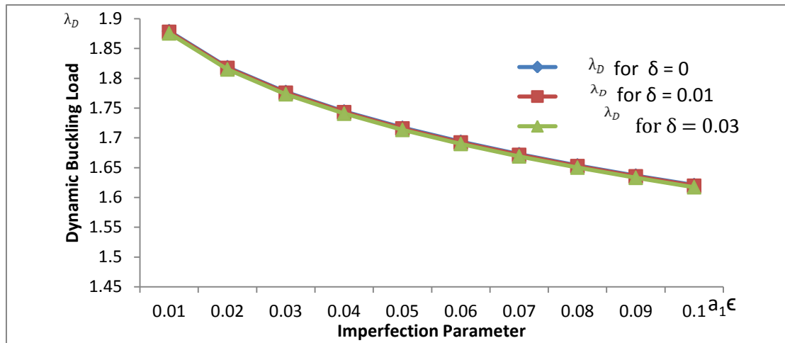
Fig. 1. Relationship between the dynamic buckling load and the imperfection parameters for different values of damping factors, using equation (4.122)
